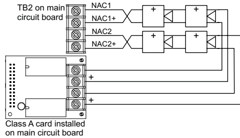
SA-CLA wiring
