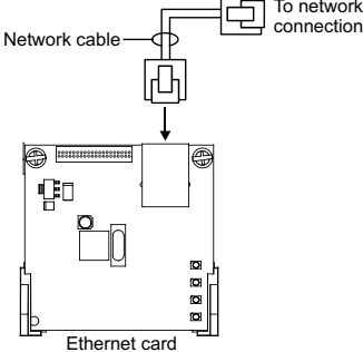
SA-ETH wiring
