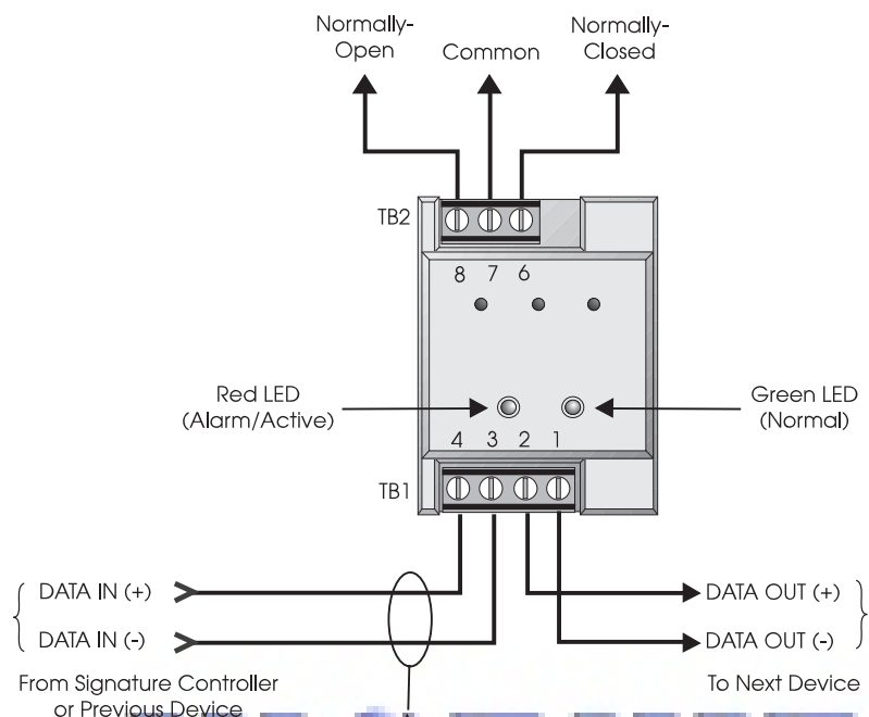
SIGA-CR Control Relay
