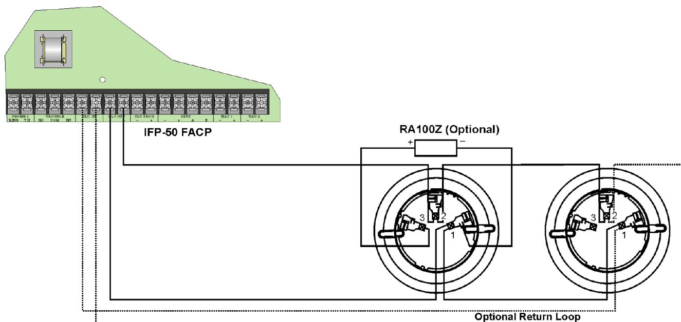
Wiring IDP-Series Detector Mounting Bases
